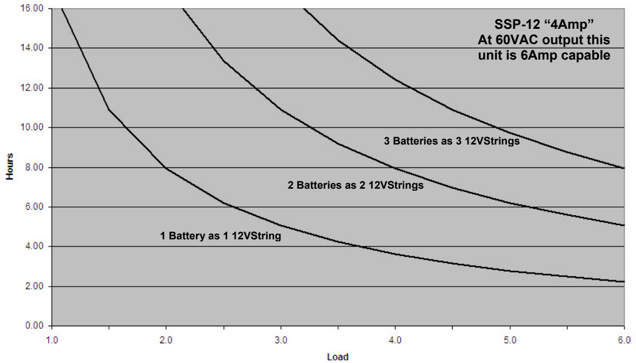
SSP-12 "4A" Battery Runtime Typical 105aH battery Output 60VAC, Load: 1 - 6 Amps
