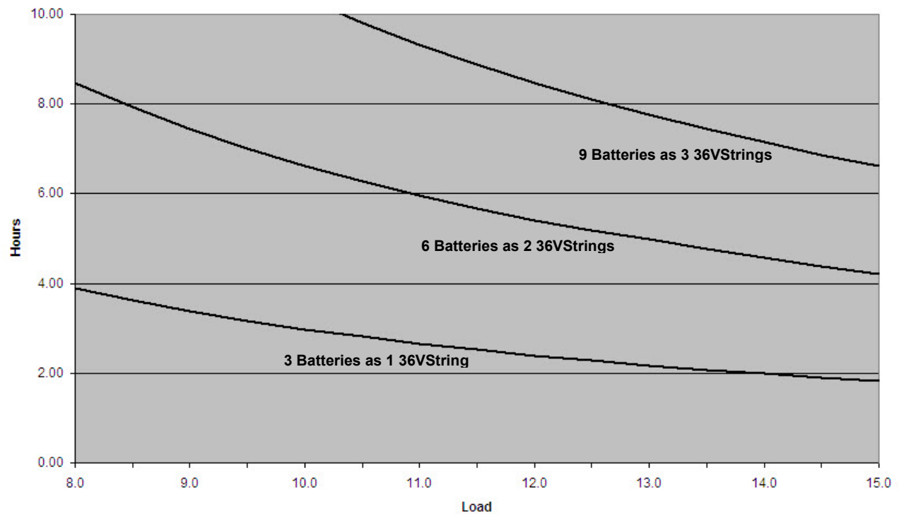
SSP-36 "15A" Battery Runtime Typical 105aH battery Output 87VAC, Load: 8 - 15 Amps
