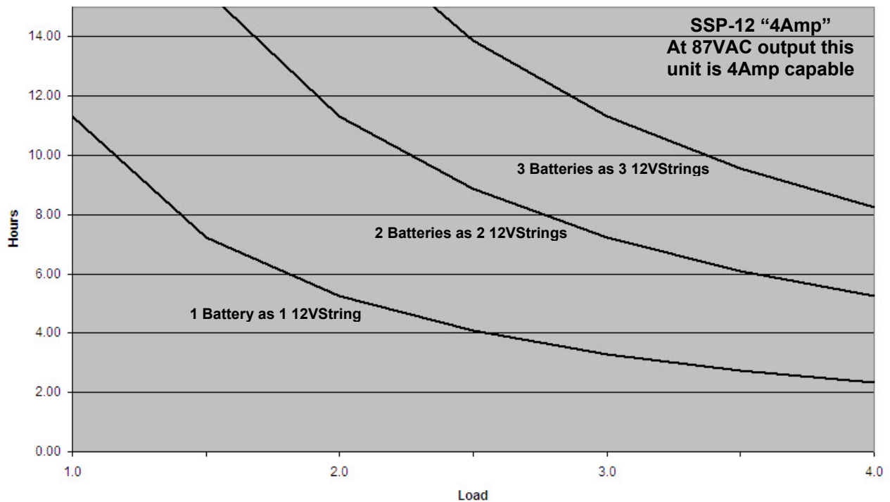
SSP-12 "4A" Battery Runtime Typical 105aH battery Output 87VAC, Load: 1 - 4 Amps
