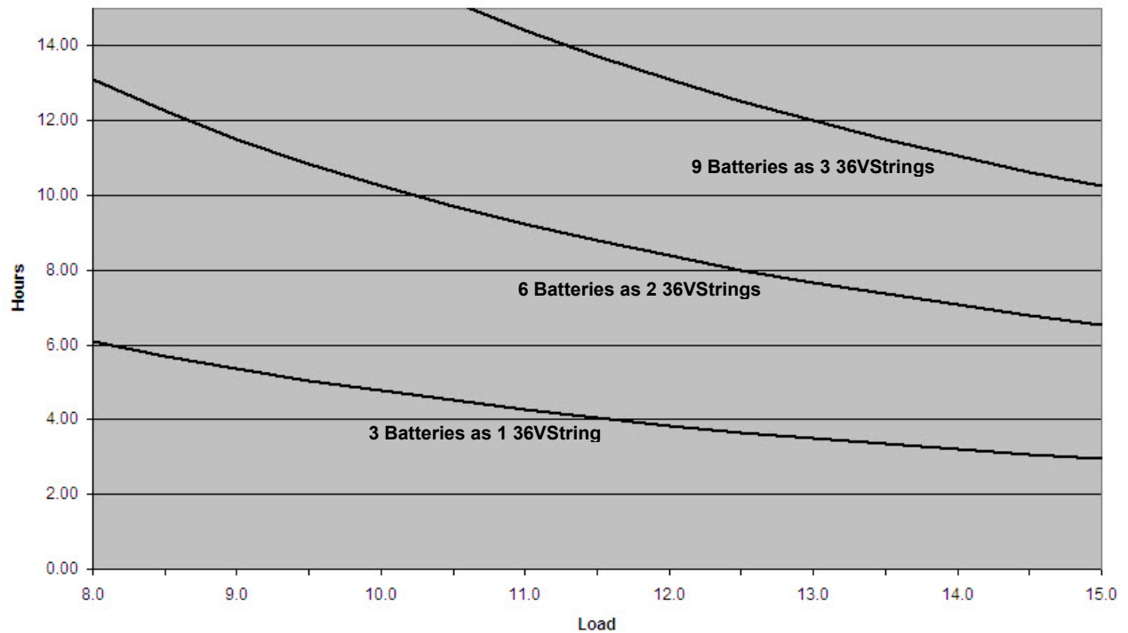
SSP-36 "15A" Battery Runtime Typical 105aH battery Output 87VAC, Load: 8 - 15 Amps
