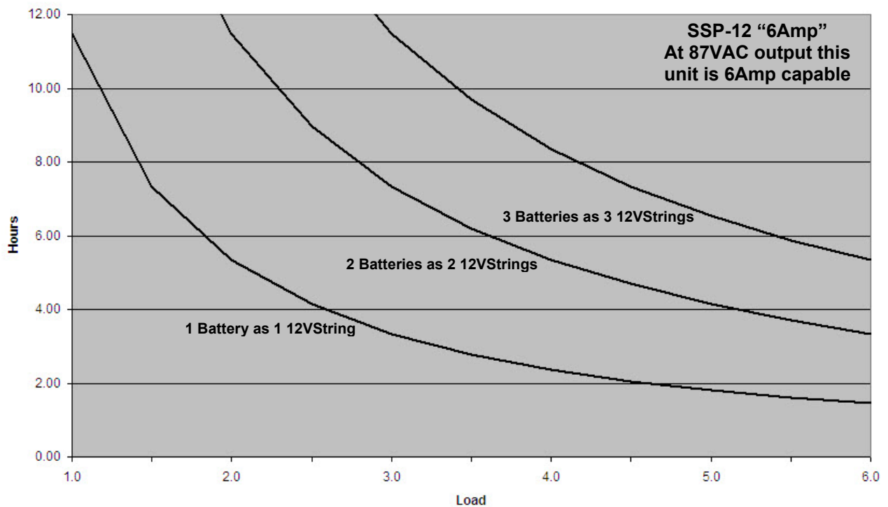
SSP-12 "6A" Battery Runtime Typical 105aH battery Output 87VAC, Load: 1 - 6 Amps
