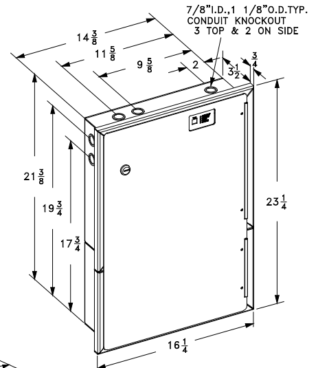
LVM 225 Wall or Recess Mount
